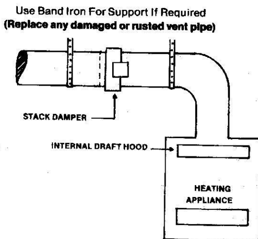
HORIZONTAL OR SLOPING INSTALLATION *
